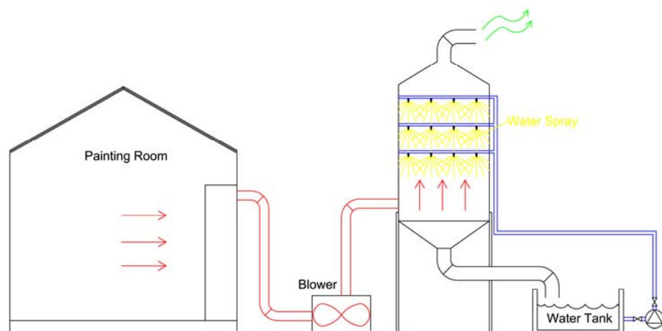
FSR Nozzle used for wet scrubber.
